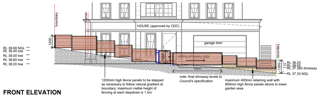
FRONT ELEVATION
