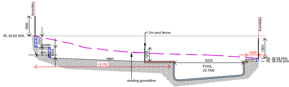
SECTION CC
